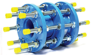
Dismantling Joint DN 100-DN 2500
